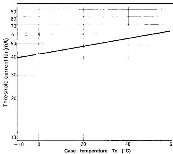
Fig. 64-3 Threshold Current vs. Temperature
