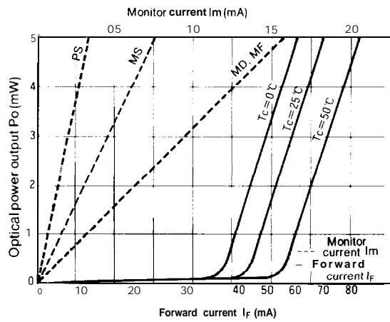
Fig. 64-2 Optical Power Output vs. Forward Current and Monitor Current
