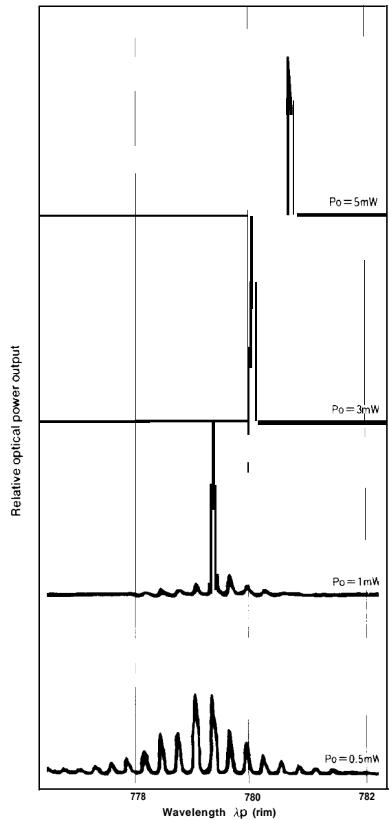
Fig. 64-5 Optical Power Output Dependence of Wavelength
