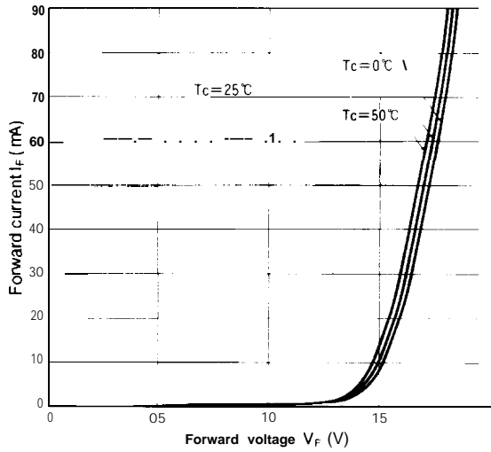
Fig. 64-1 Forward Current vs. Forward Voltage
